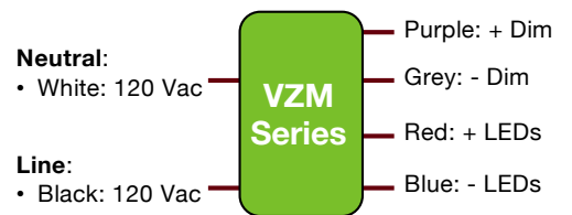
Wiring Diagram
